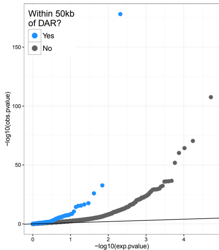
Figure S1: Differential gene expression near DARs. QQ-plot of p -values from DESeq2 analysis of gene expression for dexamethasone (A), caffeine (B), and selenium (C). The colored dots represent genes within 50kb of a DAR, while the gray dots represent genes not within 50kb of a DAR.
