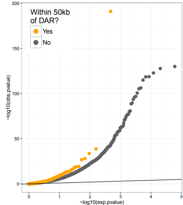
Figure S1: Differential gene expression near DARs. QQ-plot of p -values from DESeq2 analysis of gene expression for dexamethasone (A), caffeine (B), and selenium (C). The colored dots represent genes within 50kb of a DAR, while the gray dots represent genes not within 50kb of a DAR.
